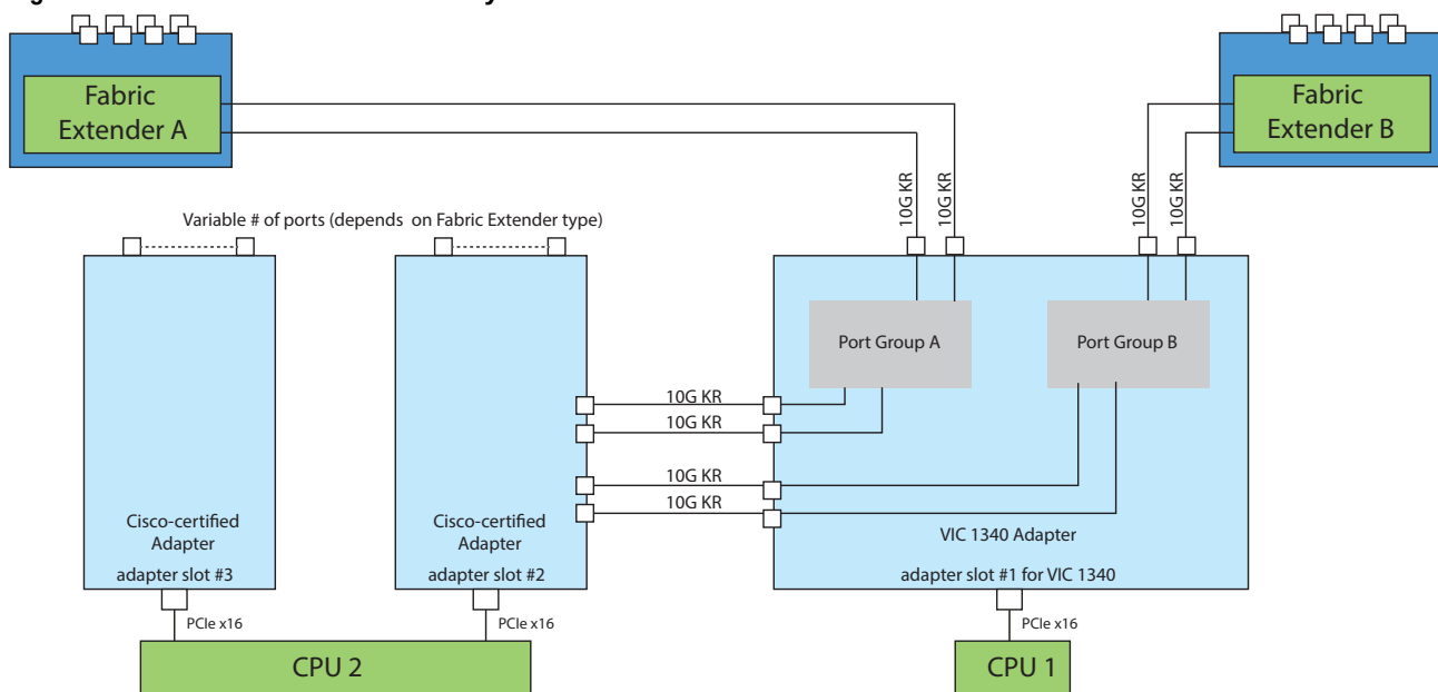
Figure 9 VIC 1340 Connectivity
