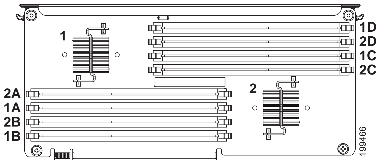
Figure 9 Memory Riser Physical Layout
