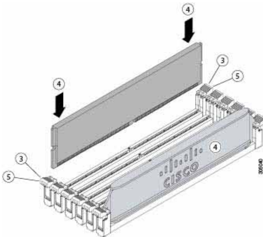
Figure 15 Replacing Memory
